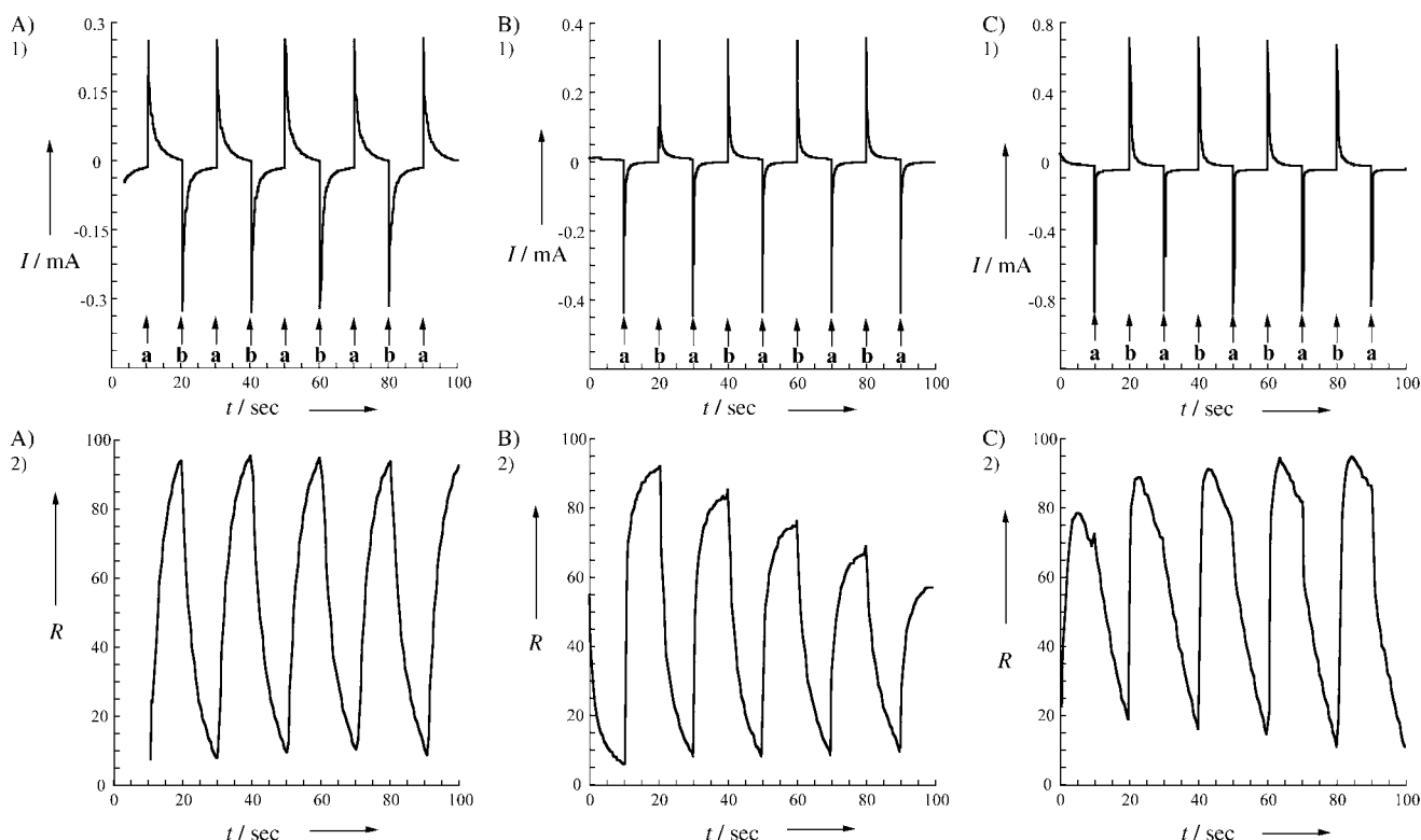
Figure 2. Multipotential step chronoamperometric transients corresponding to the transformations between A) 1) state II and state I, B) 1) state III and state II, and C) 1) state III and state I of the film. The arrows (labeled a and b) show the time of the application of the oxidative and reductive steps. Panels 2) show the time-dependent reflectance changes measured at a fixed angle of incidence at A) 2) \theta = 69.5^\circ , B) 2) \theta = 68^\circ , C) 2) \theta = 69.5^\circ upon the multipotential step experiment. The measurements were performed in 0.1 M \text{KNO}_3 , pH 7.0.
